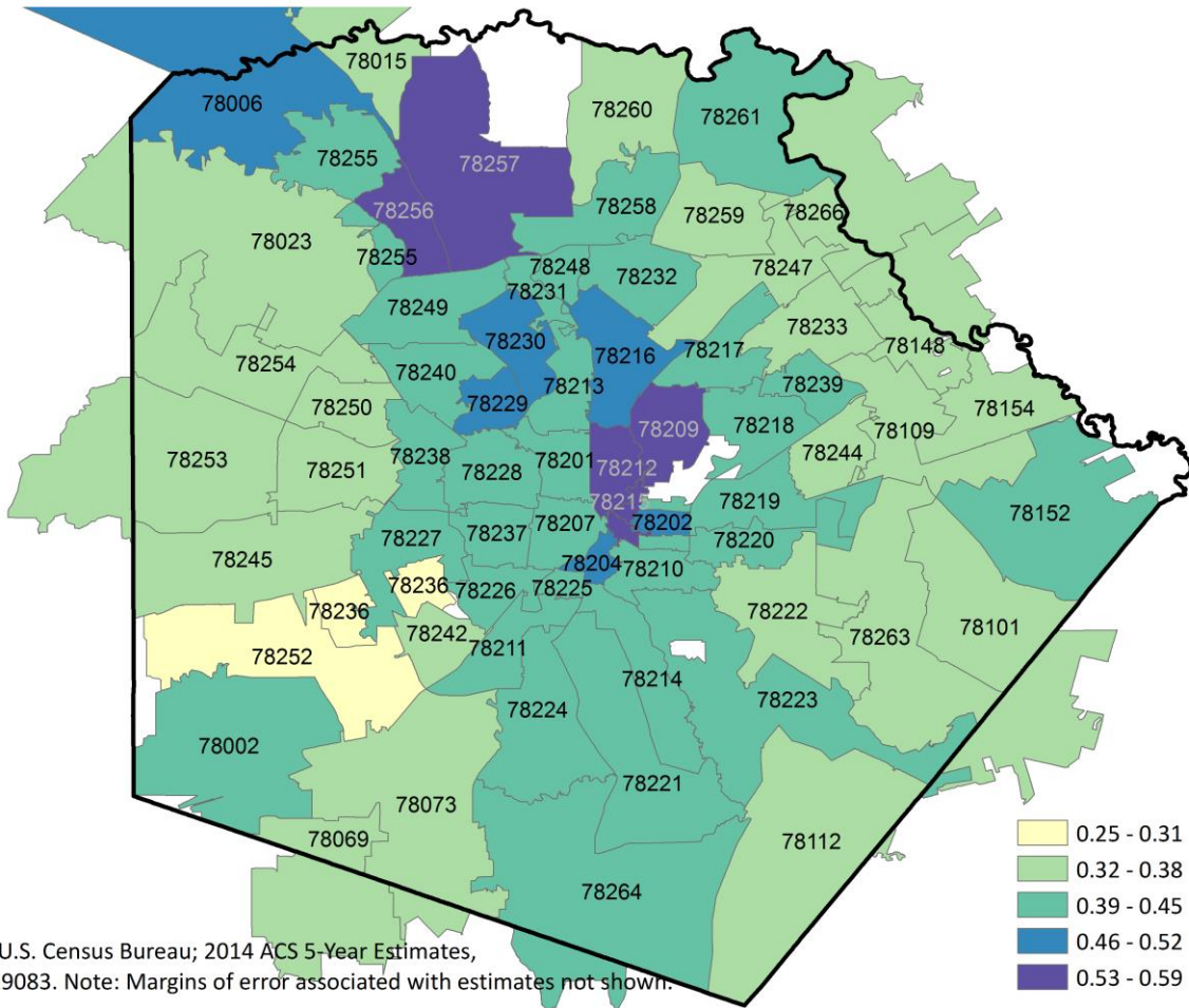
Figure 3.31 Gini Index
